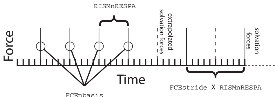
Figure 8.1.: Multiple time step methods in 3D-RISM. RISMnRESPA(=5) is the number of base time steps between application of solvation forces (exact or extrapolated). FCEnbasis(=4) is the number of previous solutions used to extrapolate forces, in this case four previous solutions. Once FCEnbasis solutions have been calculated, exact 3D-RISM forces are calculated every FCEstride(=2) \times RISMnRESPA time steps; solvation forces are otherwise obtained through extrapolation.
